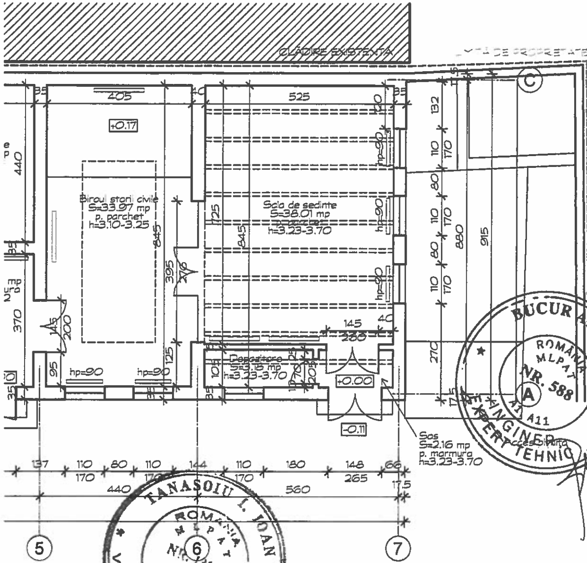
PLAN PARTER
